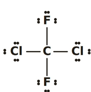
Lewis structure all formal charges 0
