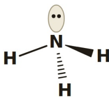
NH 3 : 107° 1 lone pair pushes the bonds closer
