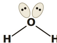
H 2 O: 104.5° 2 lone pairs push even harder
