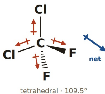
3D redraw with bond dipoles red: bond dipoles · blue: net
