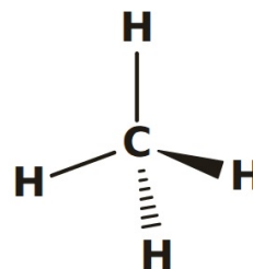
CH 4 drawn in 3D 2 in plane, 1 toward you, 1 away
